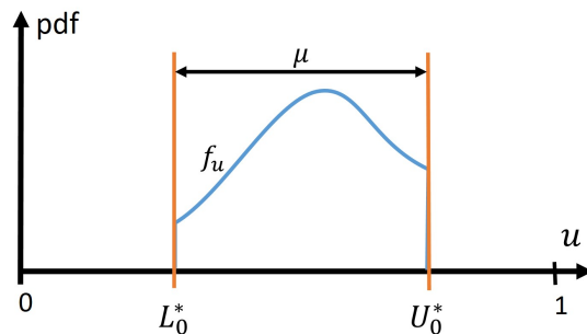
Figure 4.1: Selection of bounds L_0^* and U_0^* in case of bounded disturbance.
