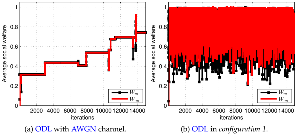
Figure 4.17: Impact of disturbances on the average social welfare for the ODL.
