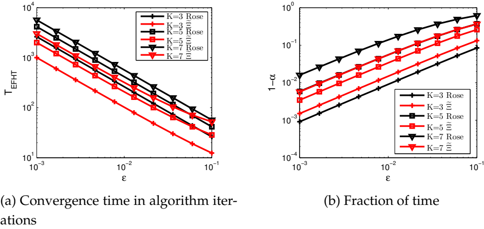
Figure 3.13: Performance comparison between our approximation and Rose approximation when N = K + 2 .
