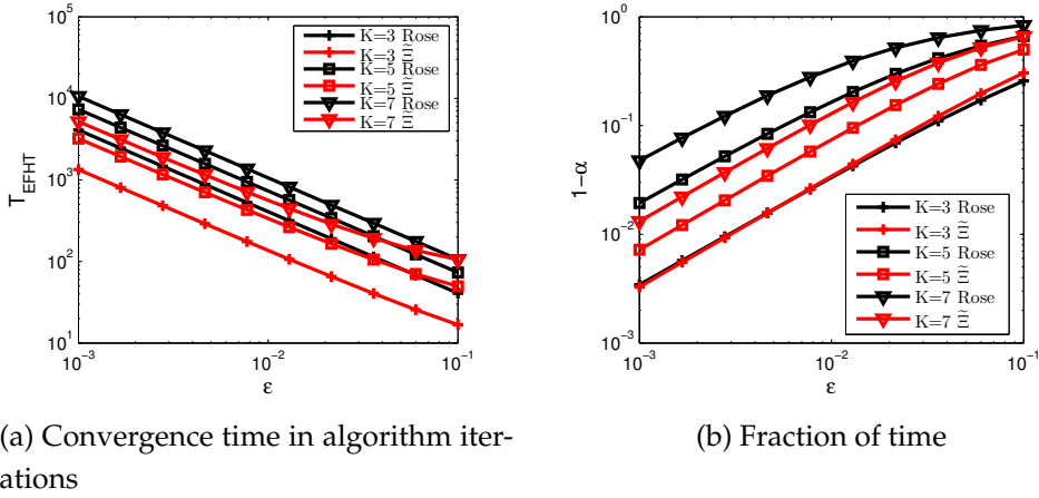
Figure 3.12: Performance comparison between our approximation and Rose approximation when N = K .
