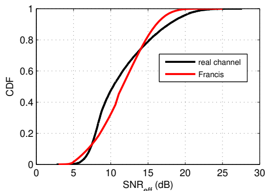
Figure 5.6: Comparison of the cdf of \text{SNR}_{\text{eff}} and \gamma_{\text{eff}} at high \gamma for N_{cc} = 50 .
