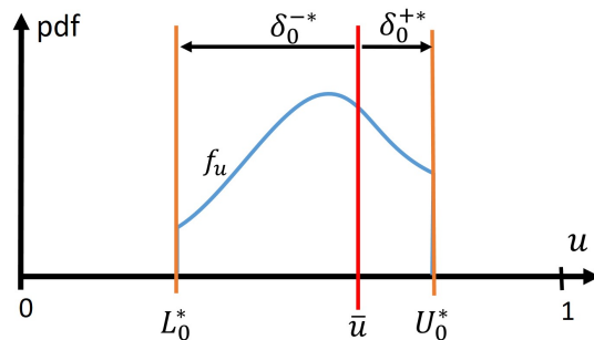
Figure 4.2: Selection of thresholds \delta_0^{-*} and \delta_0^{+*} in case of bounded disturbance.
