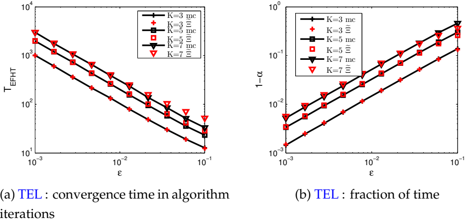
Figure 3.9: EFHT and stability comparisons between our approximated models and Monte Carlo simulations when N = K + 2 .
