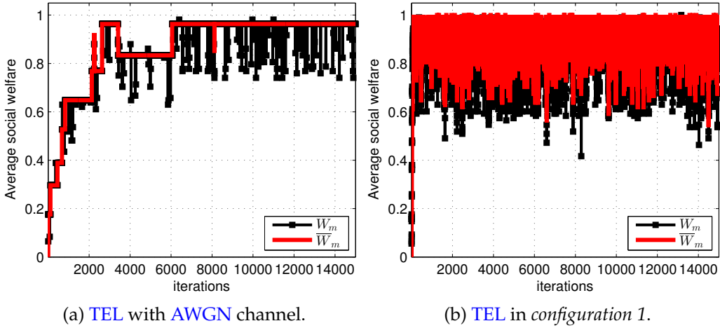
Figure 4.16: Impact of disturbances on the average social welfare for the TEL.
