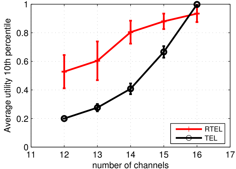
Figure 4.26: Average utility 10th percentile computed over 5 realizations of 5 clustered ad hoc networks with 12 to 16 channels in configuration 1 . Bars represent one standard deviation up and below the average value.
