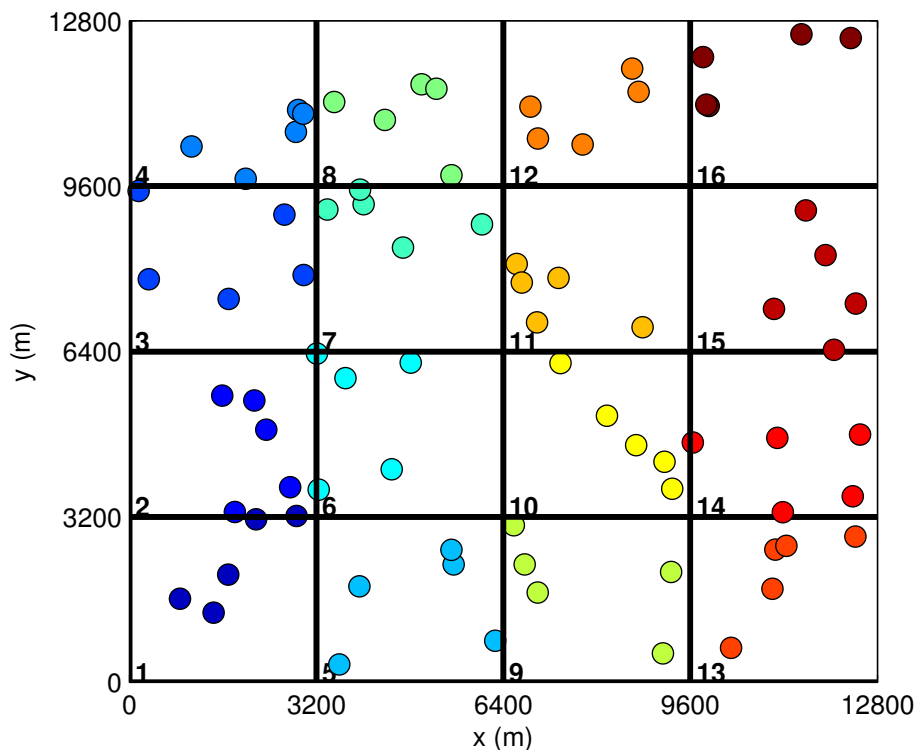
Figure 4.22: Example of a clustered ad hoc network with 16 clusters and 5 nodes per cluster. Each cluster is highlighted by square containing nodes with a specific color and an identification number on the bottom left.
