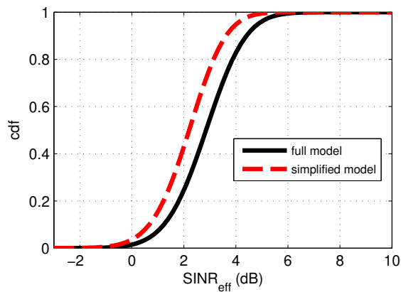
Figure 5.21: Comparison of the cdf of EESM between the simplified and full model.
