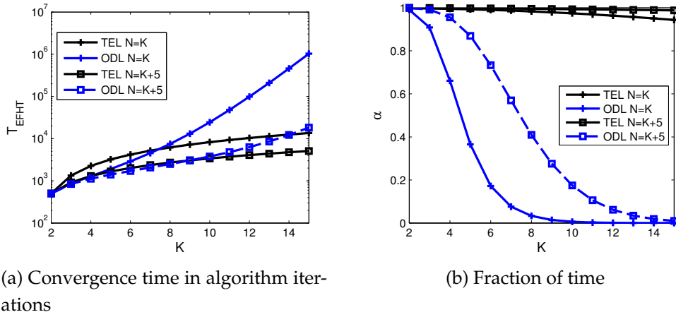
Figure 3.14: Performance comparison between TEL and ODL when \epsilon = 10^{-3} with respect to K .
