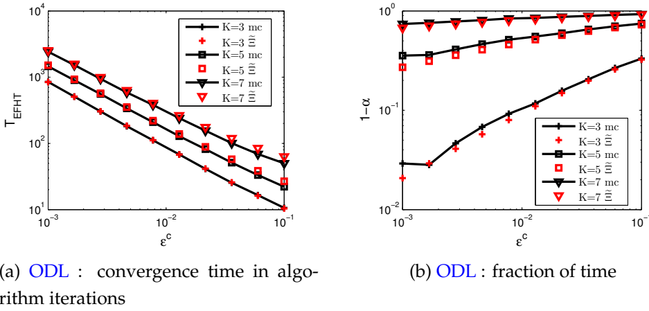
Figure 3.11: EFHT and stability comparison between our approximated models and Monte Carlo simulations when N = K + 2 .
