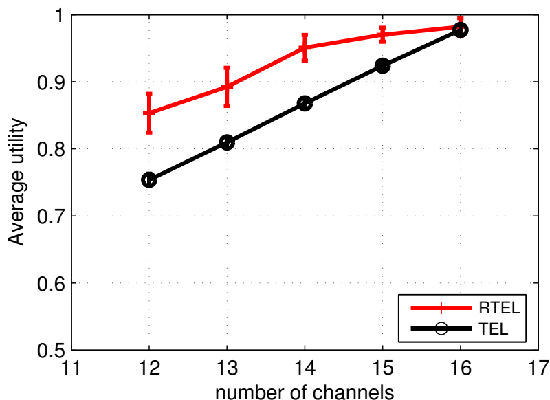
Figure 4.23: Average utility computed over 5 realizations of 5 clustered ad hoc networks with 12 to 16 channels in configuration 1 . Bars represent one standard deviation up and below the average value.
