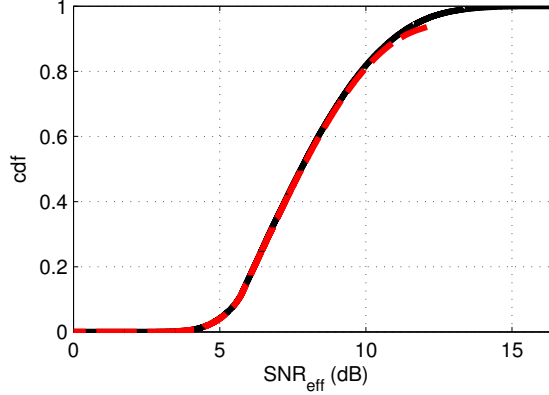
Figure 5.1: The black curve is the cdf of \gamma_{\text{eff}} obtained with Monte Carlo simulation using 10^5 realizations. The red curve is the cdf of \gamma_{\text{eff}} computed numerically with (5.26) with N_s = 1000 .
