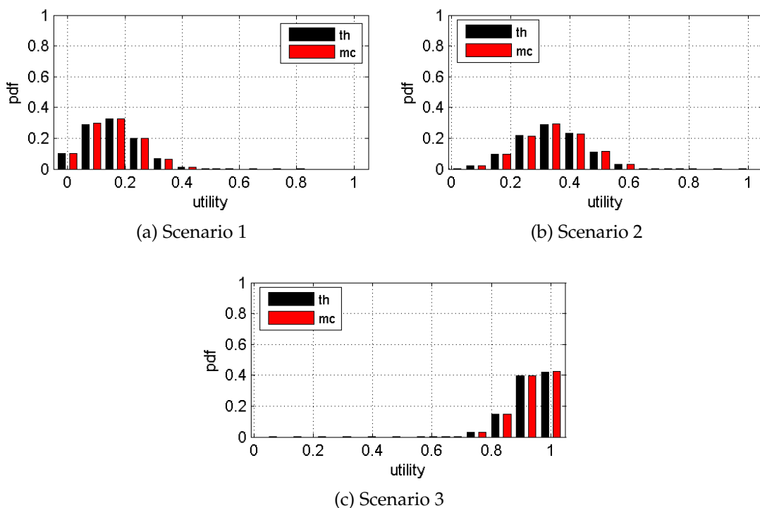
Figure 5.16: Pdf of the utility in a NB fading case.
