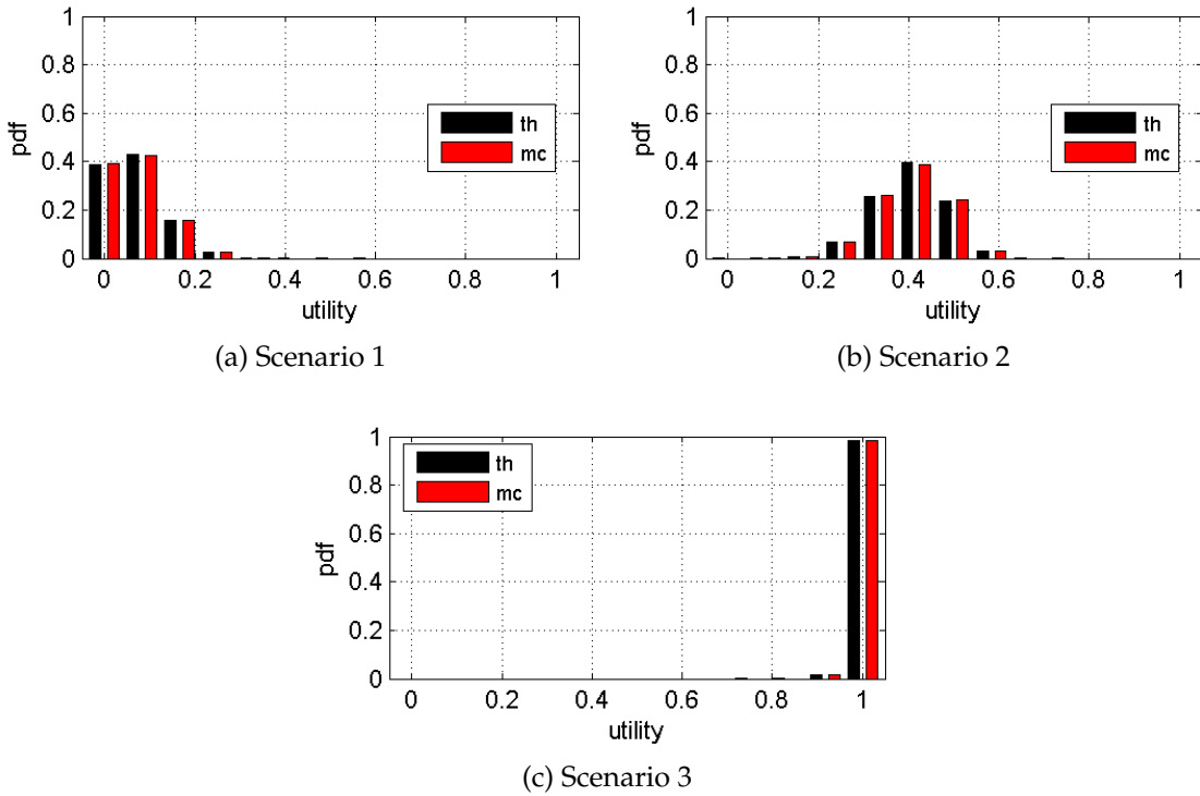
Figure 5.19: Pdf of the utility obtained when interference are subject to fading, comparison between Monte Carlo results and numerically computed results.
