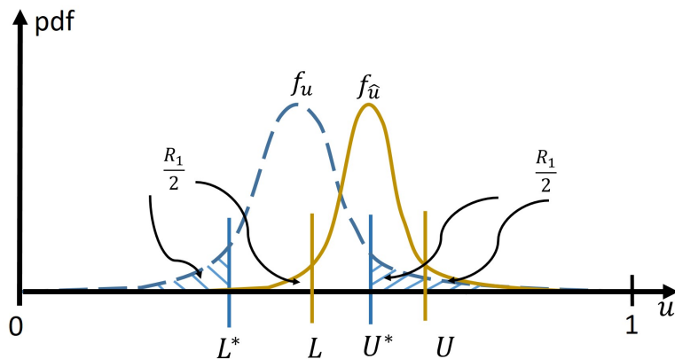
Figure 4.6: Estimation of the pdf bounds based on f_{\hat{u}} .
