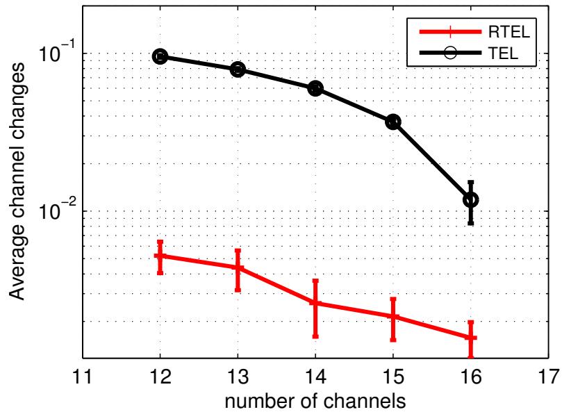
Figure 4.25: Average frequency of channel changes per cluster computed over 5 realizations of 5 clustered ad hoc networks with 12 to 16 channels in configuration 1 . Bars represent one standard deviation up and below the average value.
