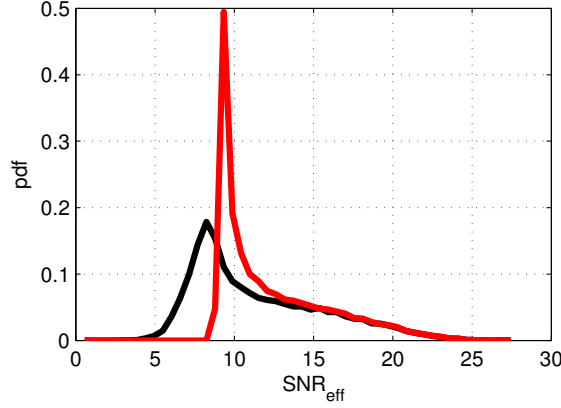
Figure 5.7: Comparison of EESM pdfs considering all terms (black curve) and the three most influential terms (red curve) into the logarithm of (5.11).
