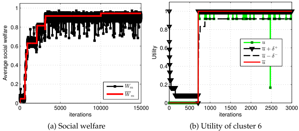
Figure 4.20: Behavior of the network with RTEL algorithm in configuration 1 .
