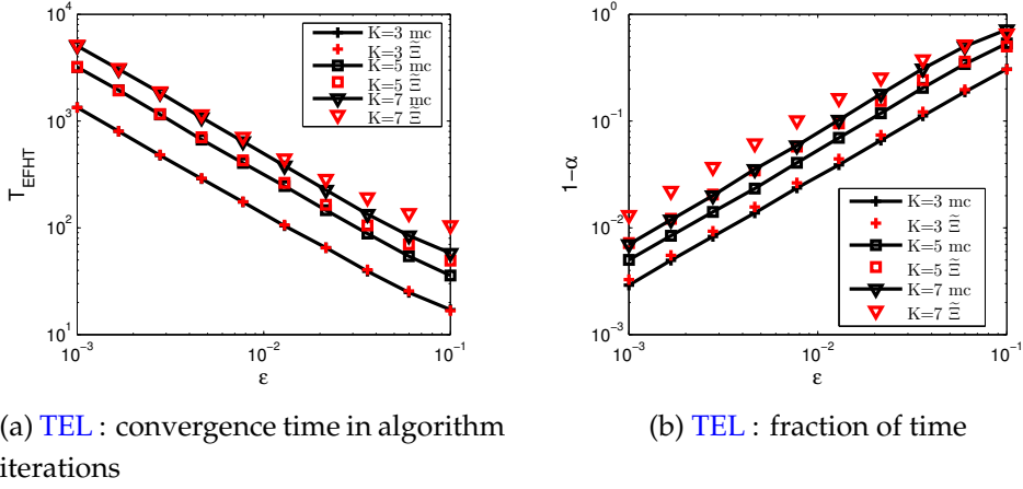
Figure 3.8: Figures of merit comparisons between our approximated models and Monte Carlo simulations when N = K .
