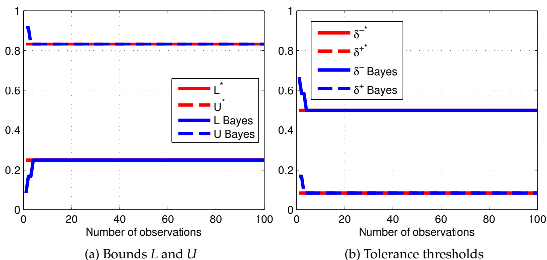
Figure 4.14: Illustration of the bounds L and U and the tolerance estimations using a Bayes method.
