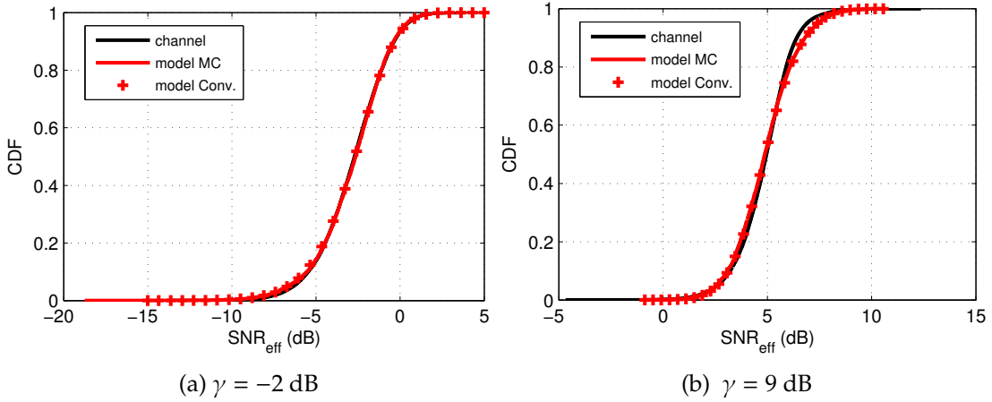
Figure 5.10: cdf comparison of EESM for different average SNR values with MCS 1.
