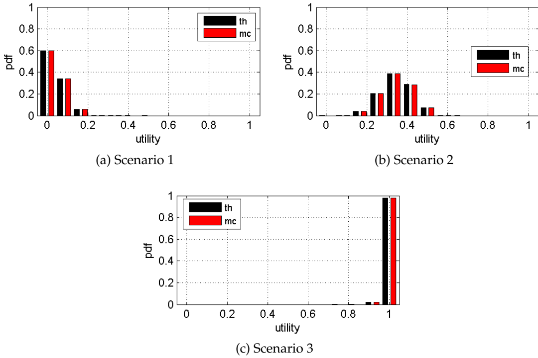
Figure 5.17: Pdf of the utility with the block fading channel (WB fading and simplified model).
