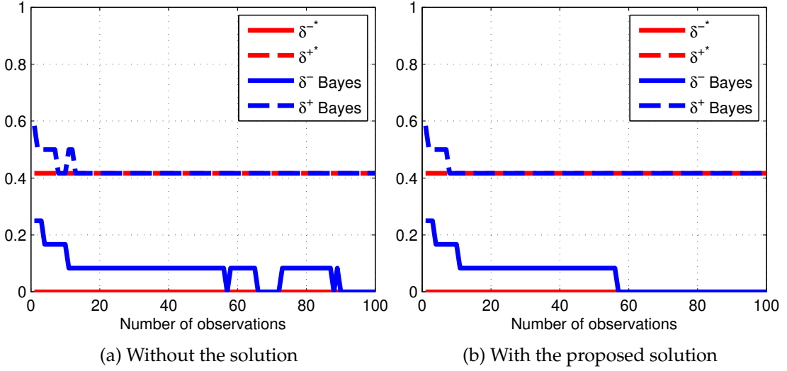
Figure 4.15: A solution to tolerance thresholds jumps.
