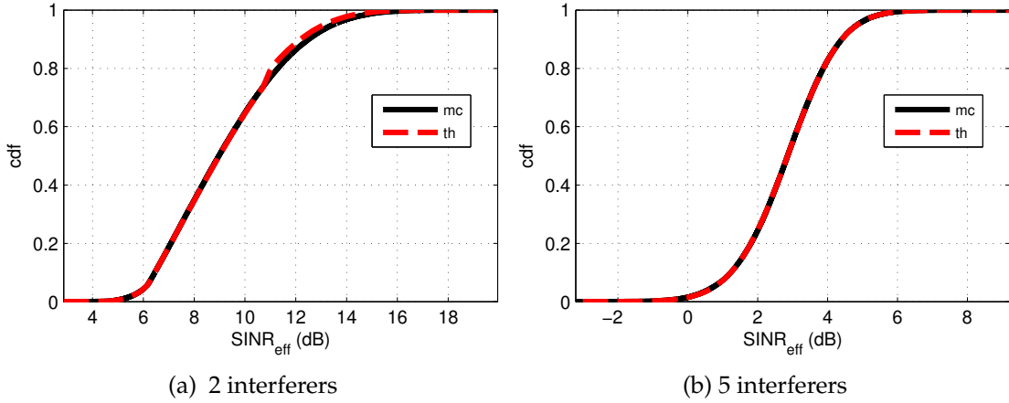
Figure 5.3: cdf of EESM when interference are subject to Rayleigh fading with different number of interferer and N_b = 10 .
