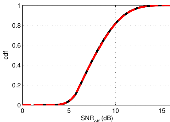
Figure 5.2: The black curve is the cdf of \gamma_{\text{eff}} obtained with Monte Carlo simulation using 10^5 realizations. The red curve is the cdf of \gamma_{\text{eff}} computed numerically with N_s = 1000 .
