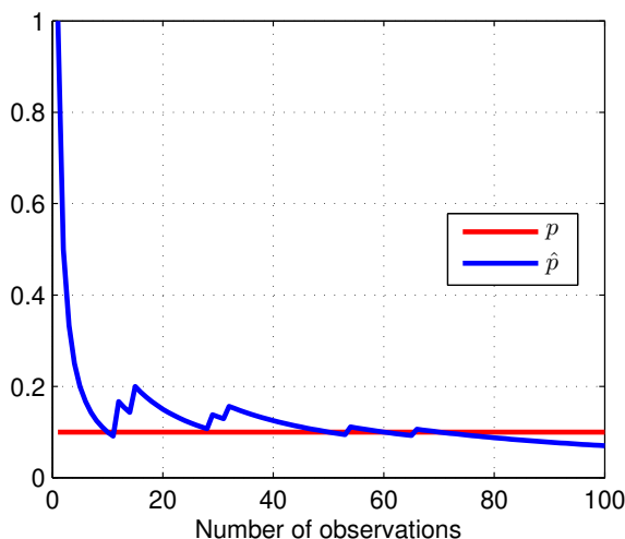
Figure 4.7: Estimation of the Bernoulli parameter using the maximum of the likelihood.
