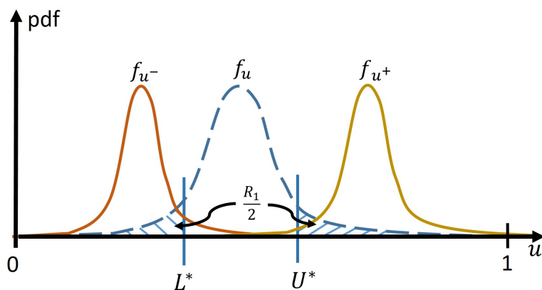
Figure 4.10: Representation of the pdfs f_{u^-} and f_{u^+} based on the Conjecture 1.
