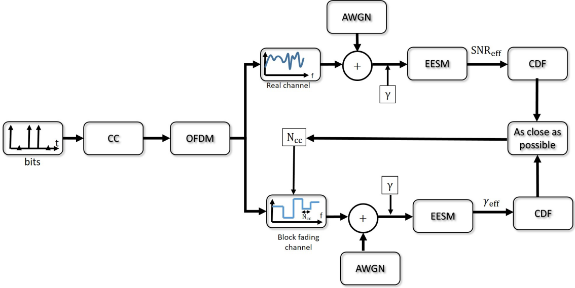
Figure 5.4: Principle of the procedure to select N_{cc} .
