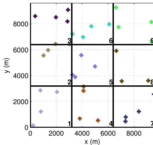
Figure 3.3: Wireless ad hoc clustered network with 9 clusters composed of 4 nodes each. Crosses represent mobile terminals, and colors the affiliations of terminals to cluster identified by the number in the bottom right of each square.
