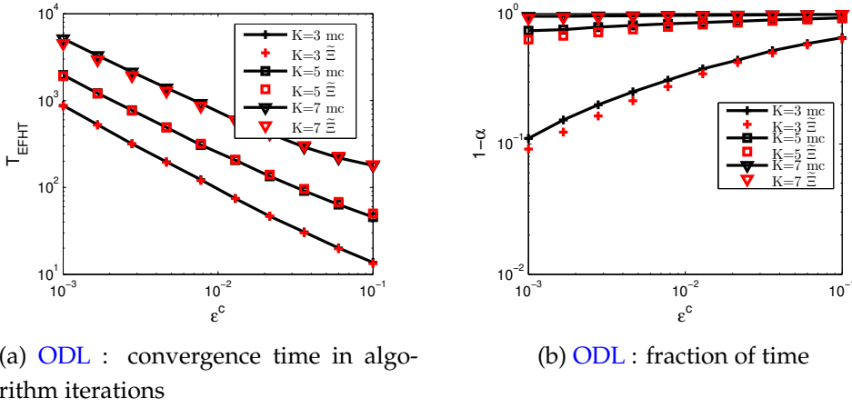
Figure 3.10: EFHT and stability comparison between our approximated models and Monte Carlo simulations when N = K .
