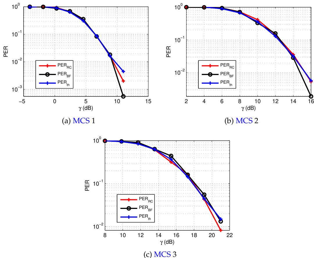
Figure 5.13: PER comparison with the channel and with the model for the three MCSs.
