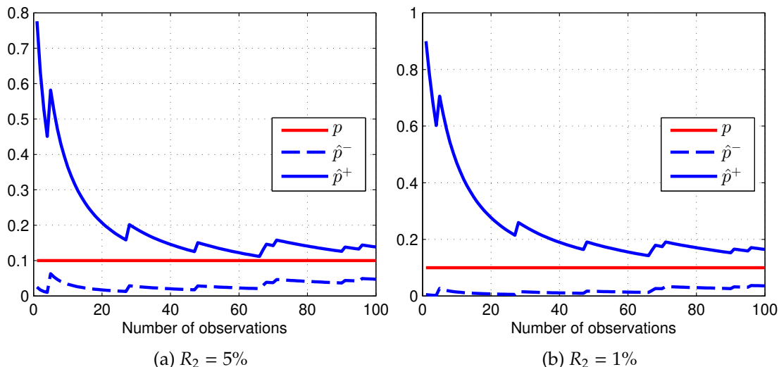
Figure 4.13: Illustration of the interval [p_i^-, p_i^+] estimation using a Bayes method.
