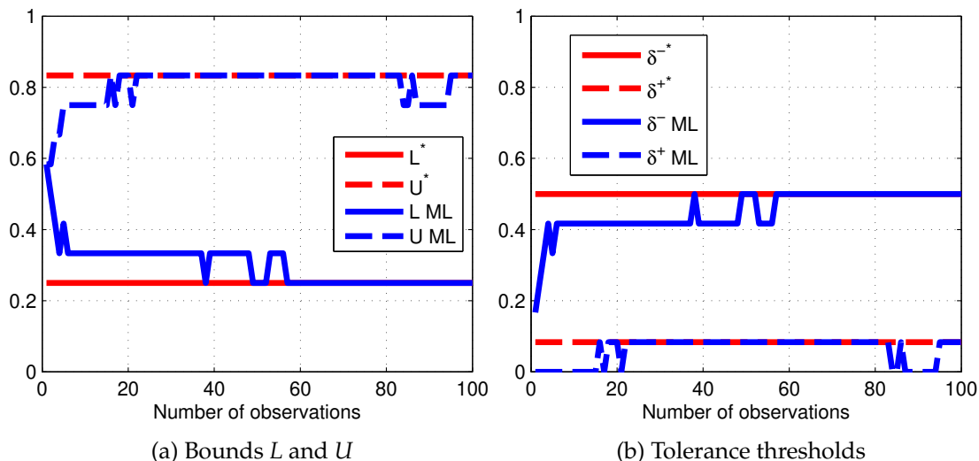
Figure 4.9: Illustration of the error estimation using a maximum likelihood procedure to compute the tolerance thresholds.
