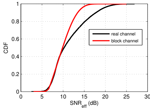
Figure 5.5: Comparison of the cdf of \text{SNR}_{\text{eff}} and \gamma_{\text{eff}} at high \gamma for N_{cc} = 20 .
