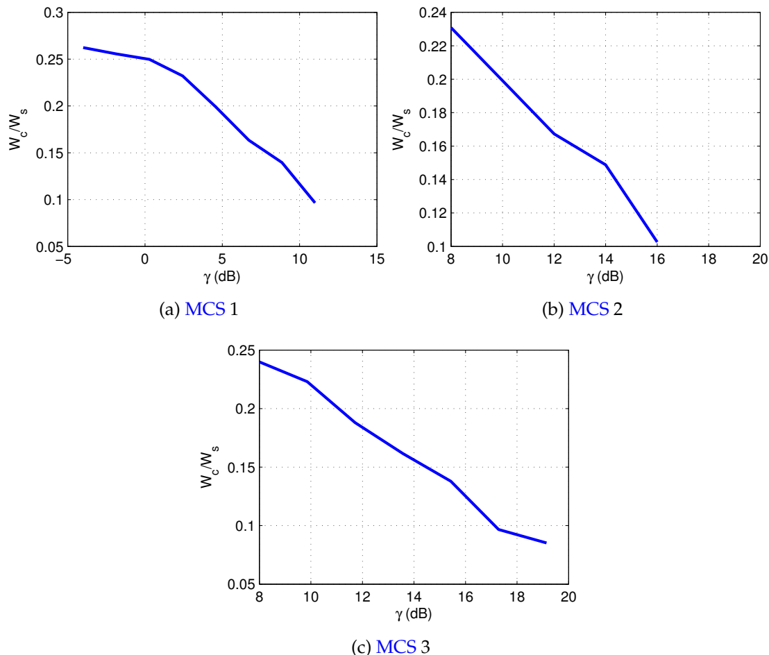
Figure 5.11: Normalized coherence bandwidth estimation using algorithm 5 with N_c = 512 .
